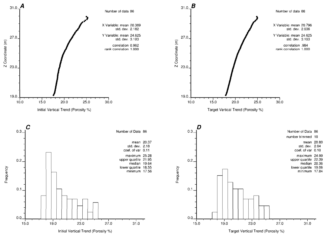
Figure 4.30: The vertical trend models: A - the initial vertical trend model from the hierarchical trend model, B - the target vertical trend based on assumed conditioning, C - the distribution of the initial vertical trend and D - the distribution of the target vertical trend. The property units are percent porosity. Note the target vertical trend has a lower variance and is more linear than the initial vertical trend.
