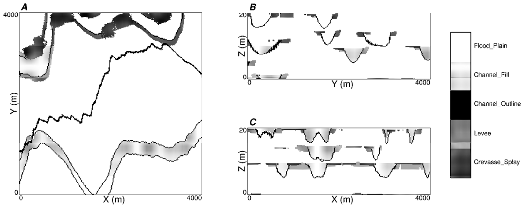
Figure 5.10: An example FLUVSIM training image - channel, levee and crevasse splay, width to thickness ratio of 100, median sinuosity and NTG of 0.2. Sections include: A - plan section, B - cross section and C - long section.
