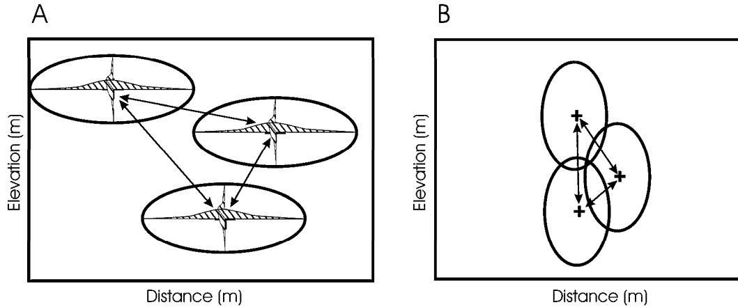
Figure 5.18: Nested associations of streamlines parameterized by mean and standard deviation of spacing between streamline associations in the vertical and horizontal and standard deviation of streamline dispersion about the centroid of the nested association. A - isolated streamline associations with a high degree of avulsion and low rate of aggradation. B - amalgamated streamline associations with high rate of aggradation and low degree of avulsion.
