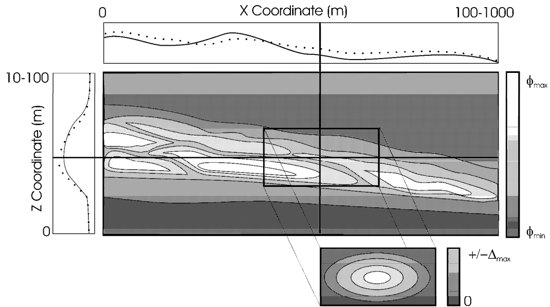
Figure 4.12: A schematic of a trend model cross section, areal and vertical, initial (dotted line) and target (solid line) trends and a multiplier window. The indicated location has a too large trend value in both the areal and vertical and so the smooth factor window is set to reduce the trend.
