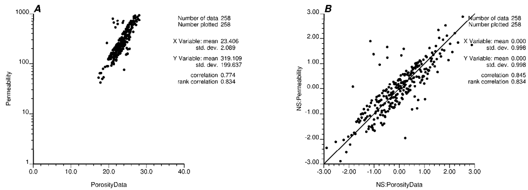
Figure 4.37: The scatter plots of synthetic well permeability and porosity, A - before Gaussian transform and B - and after Gaussian transform. The permeability is in mD and the porosity is in percent.
