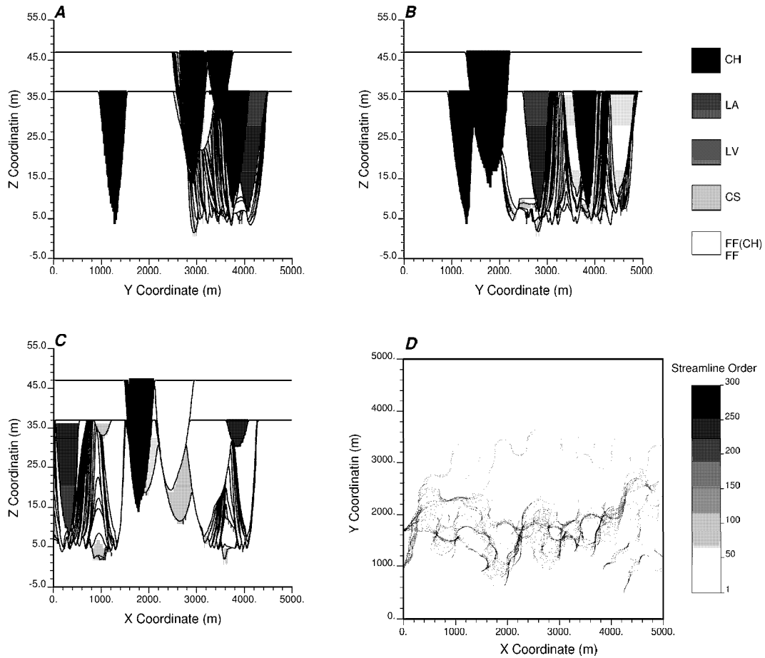
Figure 3.28: Second realization of IHS sets generated with the ALLUVSIM algorithm and parameters based on the Mossop and Flach (1983)[81] study of the McMurray Formation. A - cross section at X = 1500 meters, B - cross section at X = 4000 meters, C - long section at Y = 2500 meters and D - all of the streamlines applied to construct this model. Few streamlines were generated for visualization. In the McMurray Formation IHS sets are more extensive and FF is poorly preserved.
