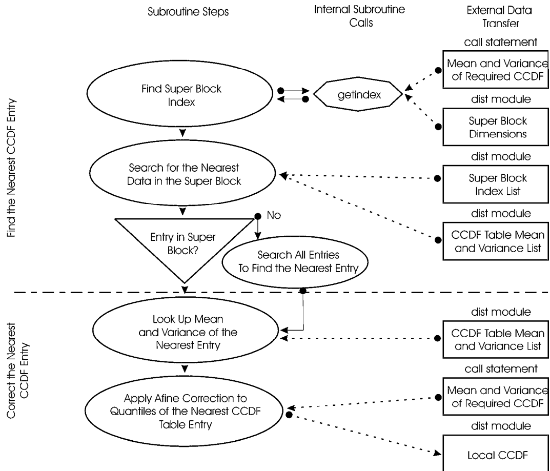
Figure 6.14: The GETCDIST subroutine flow chart. Given a required mean and variance a super block search is used to find the nearest cdf table entry. Affine correction is then applied to forced the returned cdf to have the exact mean and variance required.
