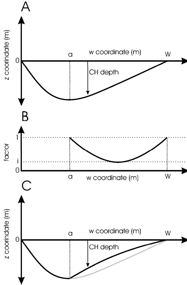
Figure 3.25: A schematic of the sigmoidal channel profile calculation. A - channel profile based on Equation 3.7. B - sigmoidal multiplier applied to CH depth. C - modified channel profile. Note a is the thalweg location and W is the channel width.
