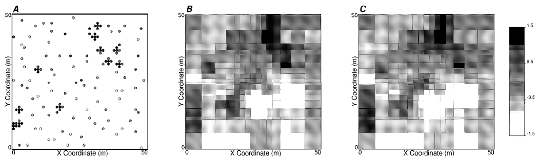
Figure 6.30: E- type estimated: A - the conditioning data locations and the e-type estimates over 201 realizations for both B - TARTANSIM and C - block averaged SGSIM.
