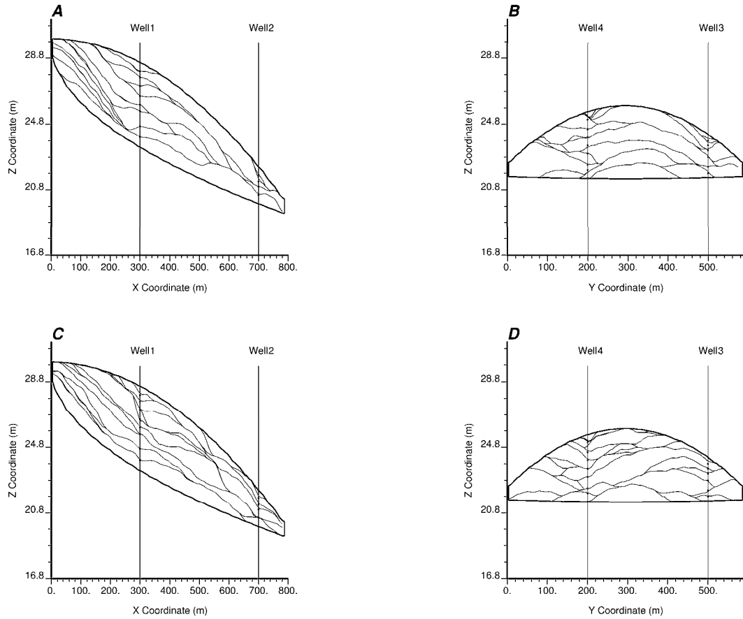
Figure 4.24: The lobe geometry, vertical well locations and sections for the demonstration of stochastic surface-based flow events within a lobe: A - first realization long section A - A' , B - first realization cross section B - B' , C - second realization A - A' and D - second realization cross section B - B' long section.
