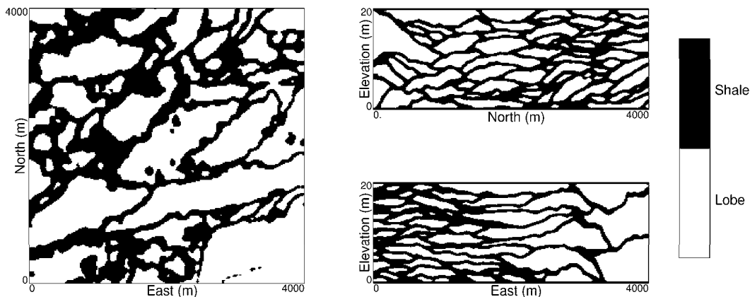
Figure 2.6: An example surface based simulation. Cross sections have \times 75 vertical exaggeration. Note a stratigraphic transformation was applied to set a constant thickness. The actual feature thins towards the southeast.
