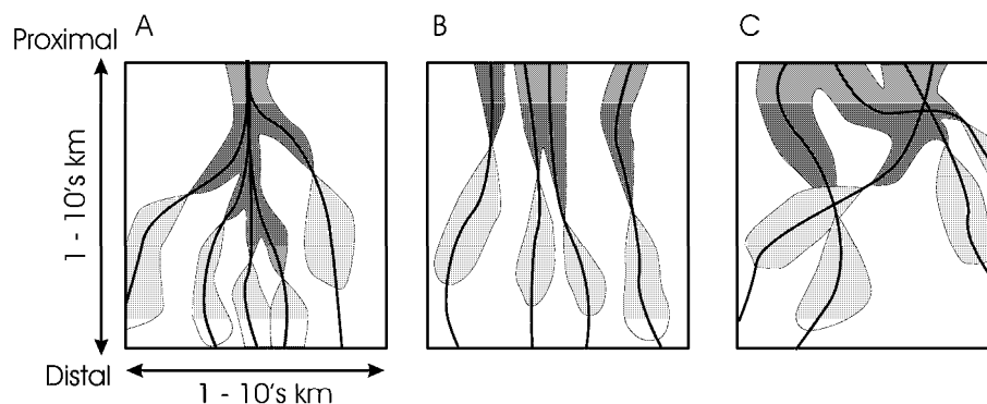
Figure 5.22: The influence of source and primary azimuth distribution on streamline associations: A - point source canyon, B - line source, shelf edge and C - delta front (Hobday and Galloway, 1996)[41]. All views are plan sections.
