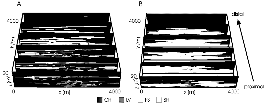
Figure 5.23: Cross sections of two example channelized sheet complex training images. A - apron source, high frequency of branching and thin SH elements and B - point source, low frequency of branching and thick SH elements.
