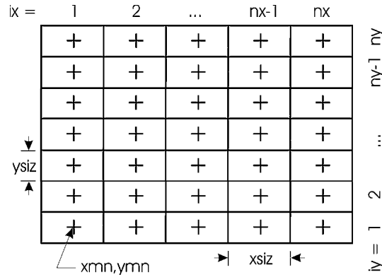
Figure 6.4: An example regular Cartesian grid and the associated parameters. This schematic is based on Figure II.1 from Deutsch and Journel, 1998.[24]
