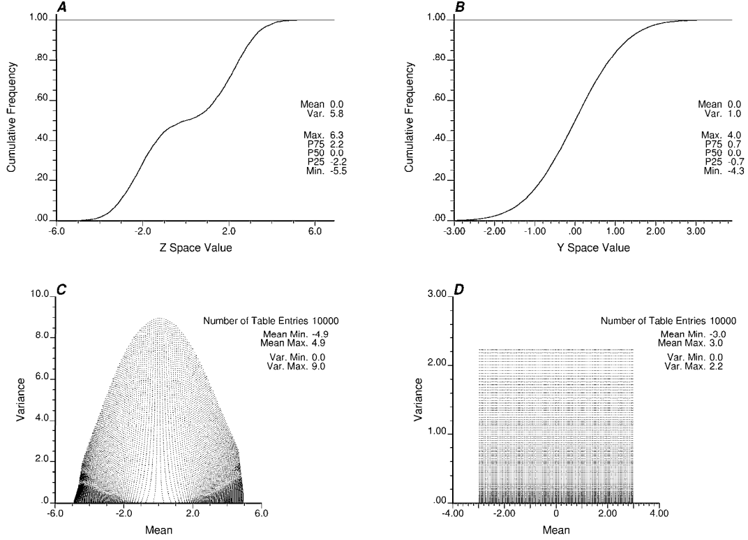
Figure 6.9: Example Y and Z global distributions and the resulting ccdf table entries. A - the Z space reference distribution is set as a bimodal distribution and B - the Y space is the required standard normal distribution. D - the regular series of means and variances for which local distributions were calculated are shown along with C - the resulting means and variances of the Z space entries.
