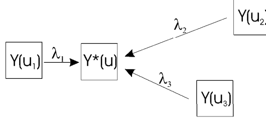
Figure 2.3: An example estimation problem. Y is the RF with any nonstationary trend, m(\mathbf{u}) , removed, Y(\mathbf{u}) = Z(\mathbf{u}) - m(\mathbf{u}) .
