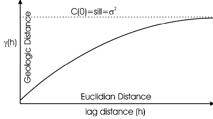
Figure 2.2: A schematic of a semivariogram model. The semivariogram quantifies the relationship between Euclidian distance and geologic distance or change.
