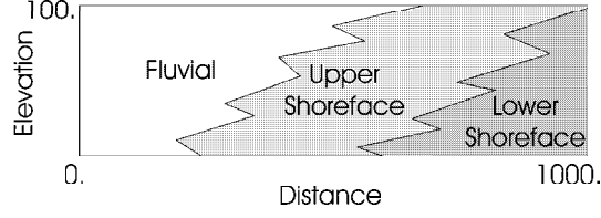
Figure 2.4: A schematic of a prograding coastal setting where facies ordering is an important feature. Facies include from fluvial sands, upper shoreface sands and lower shoreface sands. Units are in meters.
