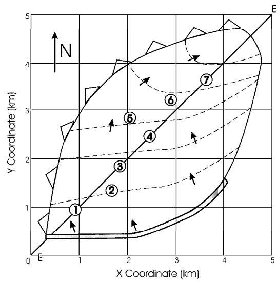
Figure 4.35: A schematic of the initial bathymetry loosely based on a study of Cengio turbidite system Italy (Cazzolo et al., 1985)[14]. The dark gray section represents the source for flow events. The fan lobe onlaps a mudstone slope along the west, northwest and north. The vertical well locations and the paleocurrents are indicated. The study area is 25 square kilometers.
