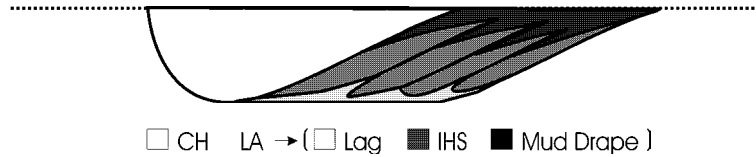
Figure 3.24: A schematic dip section of the morphology of IHS sets associated with meandering fluvial systems. Adapted from Thomas et al. (1987)[132]. Compare to the architectural element model in the ALLUVSIM algorithm (see Figure 3.8).
