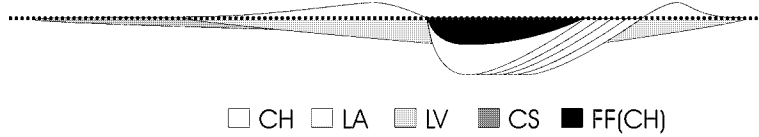
Figure 3.8: An illustration of the fluvial architectural elements applied in the stream-line based model.
