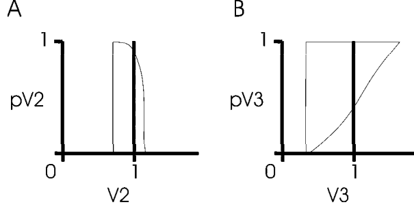
Figure 4.9: Example porosity (units relative to the global mean) vertical trend functions for: A - 2^{nd} and B - 3^{rd} hierarchical orders. Note they each have distinct shapes. Since the 3^{rd} order has greater variability it will have more influence on the final composite trend model. These vertical trends are similar to vertical turbidite lobe trends identified by Stow et al. (1996)[124].
