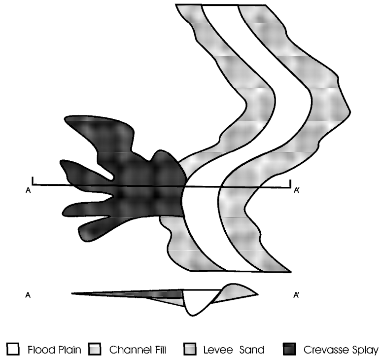
Figure 5.7: A schematic of the FLUVSIM model (based on Deutsch and Tran (2002)[26]).
