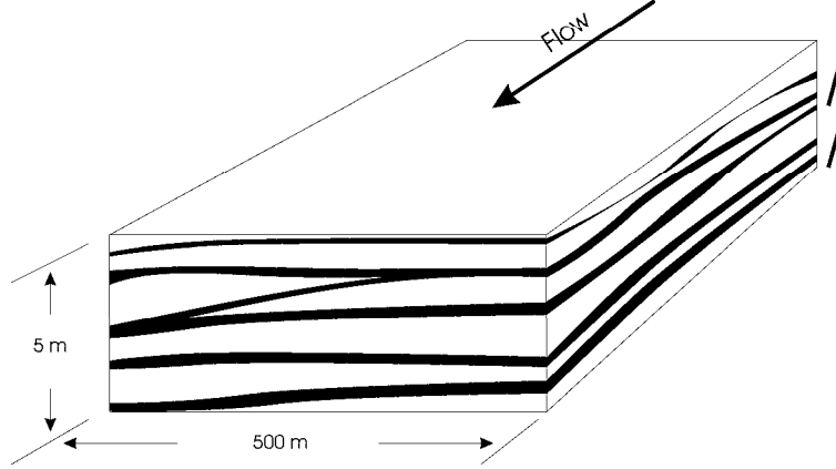
Figure 4.2: A drawing similar to the schematic illustration of compensational bedding from Mutti and Sonnino (Figure 2, 1981)[84].
