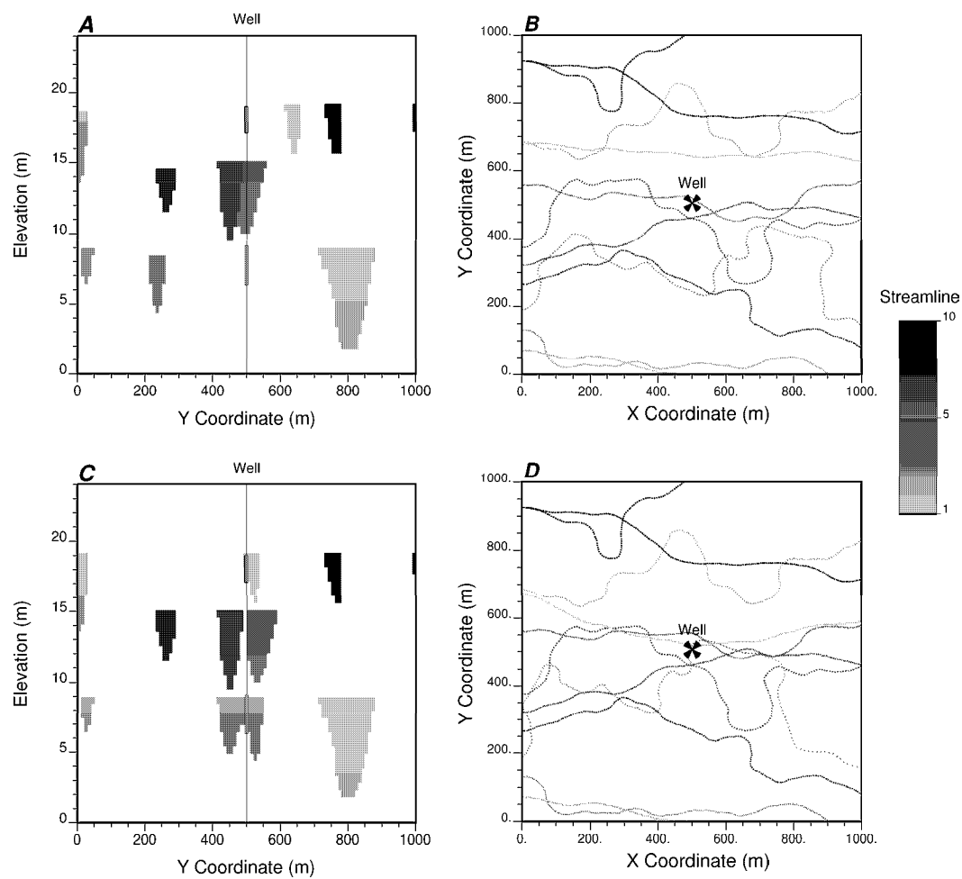
Figure 3.23: An example conditional streamline based model from ALLUVSIM.
