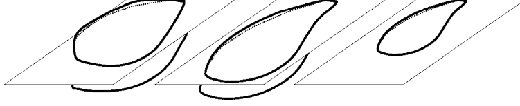
Figure 4.17: Three example candidate surfaces based on the lobe surface template in Figure 4.16. The length and width are varied. Note the surfaces are shown truncated by a plane.
