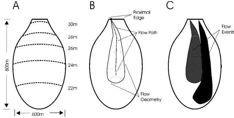
Figure 4.21: The construction of individual flow events within a lobe: A - a lobe geometry and bathymetry are defined, B - a stochastic flow events are generated, characterized by flow path and flow geometry and C - subsequent flow events are generated until the lobe is filled.
