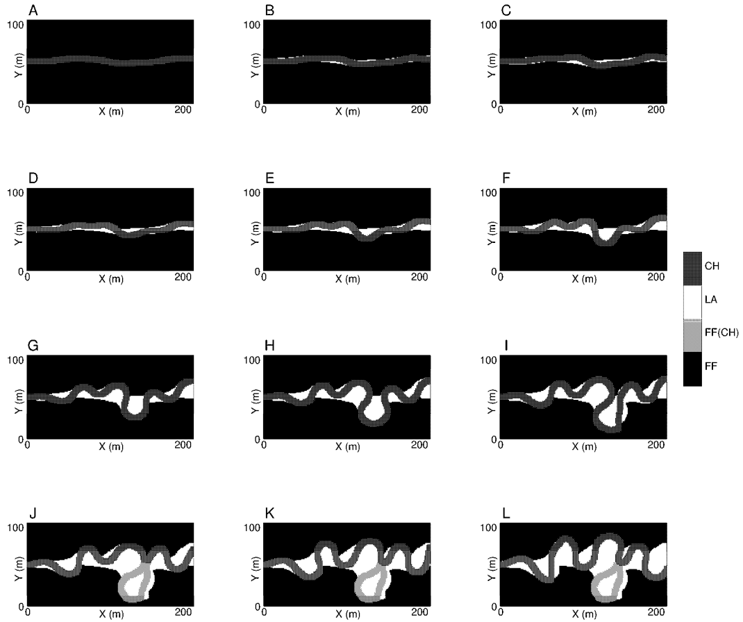
Figure 3.6: The migration of a channel streamline over twelve time steps and the evolving facies model. A to L - note the formation of LA elements and increasing streamline sinuosity. J - a neck cutoff occurs and the oxbow lake is coded as abandoned channel fill (CH element capped with FF(CH) element).
