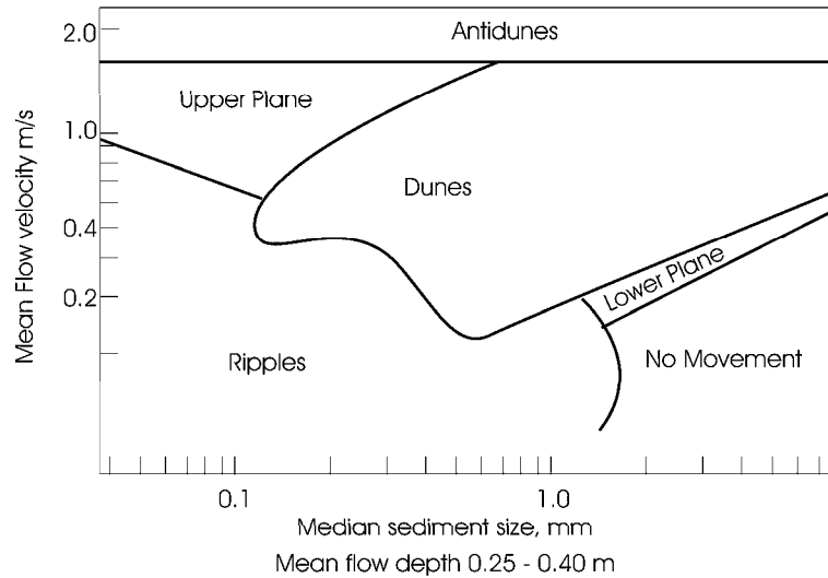
Figure 3.1: A schematic of mean flow velocity vs. median sediments size and the stability fields for difference sand beds (adapted from Miall, 1996)[78]
