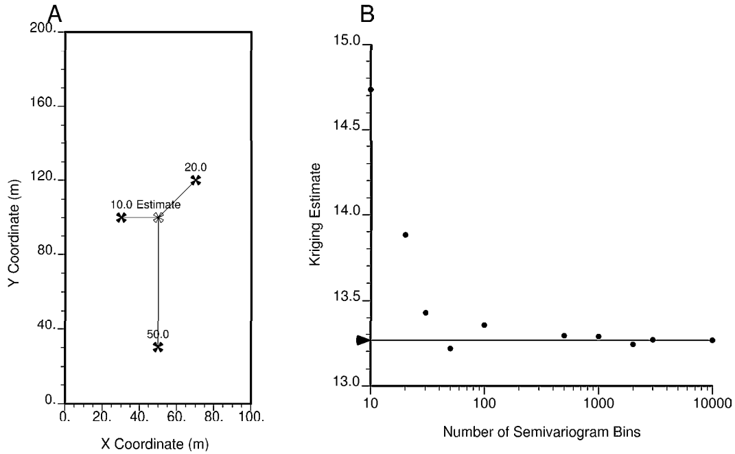
Figure 6.11: An example to demonstrate the sensitivity of kriging estimate to the number of bins in the semivariogram look up table. A - the conditioning data and estimate location. An isotropic spherical semivariogram with a range of 100 meters was applied. B - the kriging estimates with respect to the number of bins in the semivariogram look up table. The kriging estimate based on the actual semivariogram values is indicated by the horizontal line.
