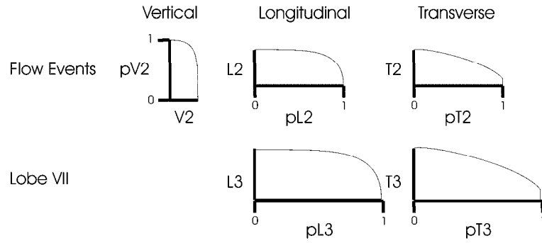
Figure 4.41: The porosity trends inferred from the lithofacies study of the Cengio Turbidite System, Italy (Cazzolo et al., 1985)[14]. The flow events have subtle grading and are often capped by fine grained facies. Flow events and the lobes demonstrate an increase in fine facies towards the distal and are coarsest along the primary axis of flow.
