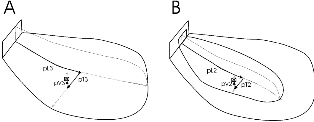
Figure 4.8: A demonstration of the depositional coordinate system describing vertical, longitudinal and transverse location within nested architectural elements (A - lobe scale and B - flow event scale). The striped section represents the primary flow axis at each scale.
