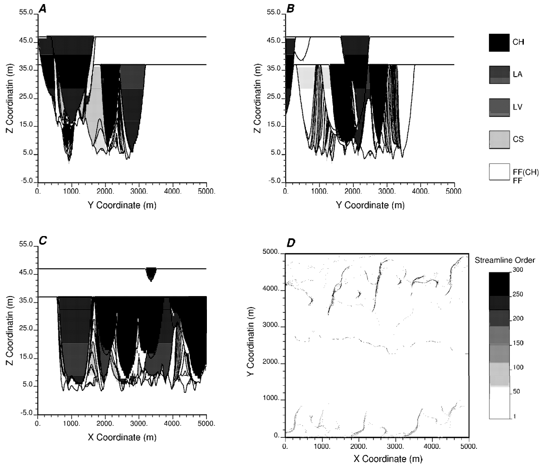
Figure 3.27: First realization of IHS sets generated with the ALLUVSIM algorithm and parameters based on the Mossop and Flach (1983)[81] study of the McMurray Formation. A - cross section at X = 1500 meters, B - cross section at X = 4000 meters, C - long section at Y = 2500 meters and D - all of the streamlines applied to construct this model. Few streamlines were generated for visualization. In the McMurray Formation IHS sets are more extensive and FF is poorly preserved.
