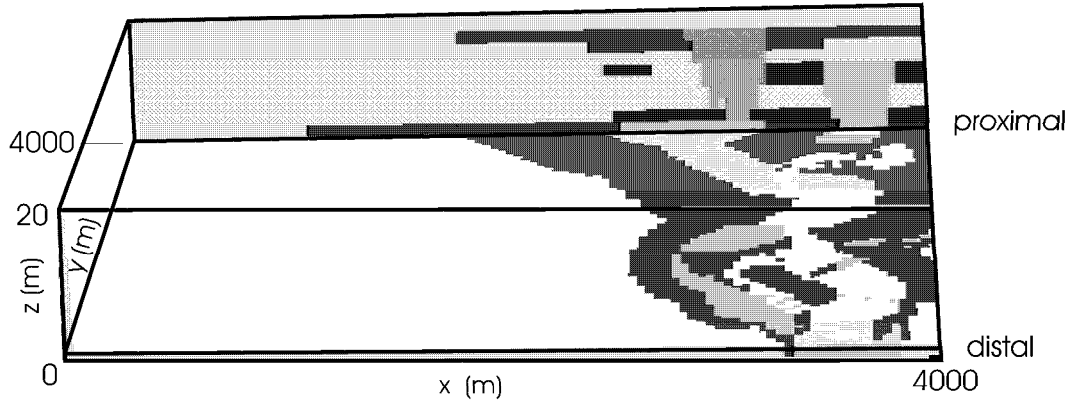
Figure 5.20: Example channel and levee complex training image. There are two streamline associations stack on top of each other. The CH elements have a mean width of 400 meters and a sinuosity of 1.3. The LV elements have a nominal width of 500 meters and a LV thinning factor of 1.0.
