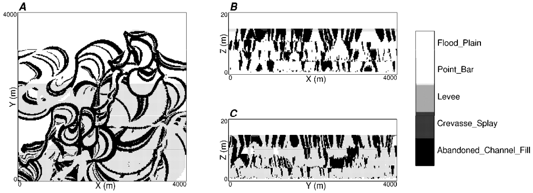
Figure 5.27: Example training image for the inference of statistics. A - plan, B - long section and C - cross section. Note the alternating coarse and fine grained channel fills.
