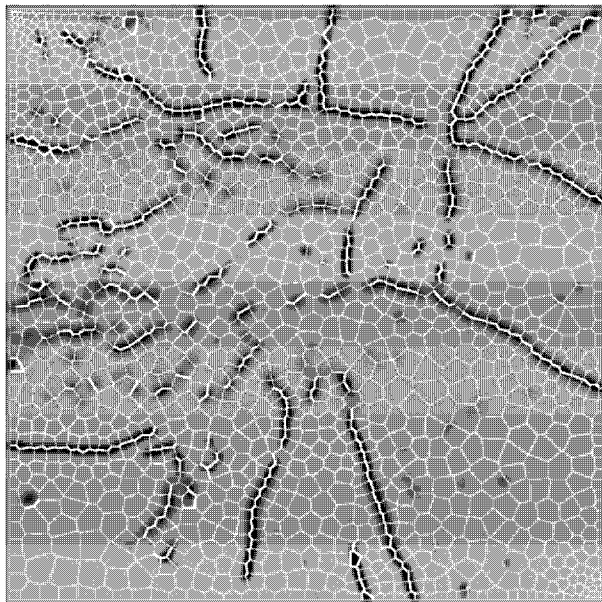
Figure 6.35: An atomic grid provided by D. Hale, Landmark Graphics (2002)[48].
