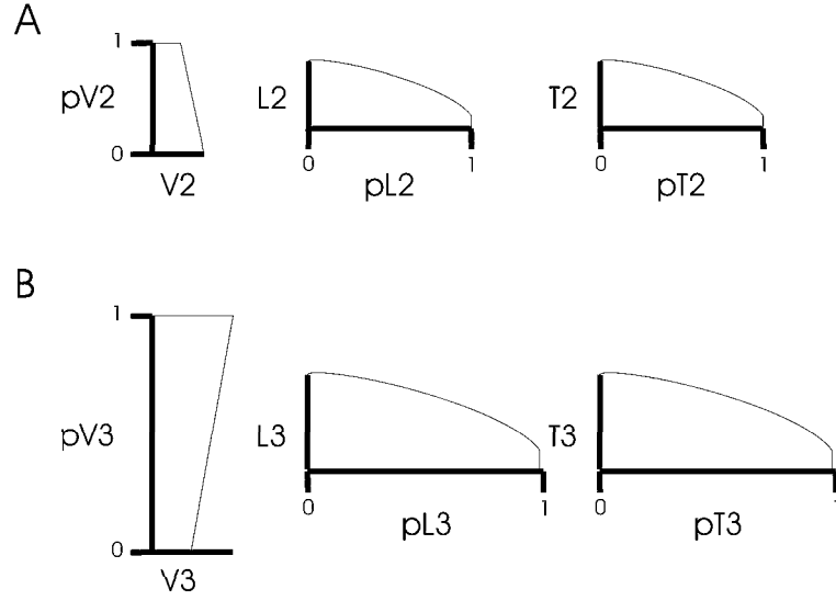
Figure 4.10: A potential suite of porosity trends that may be applied in the vertical, longitudinal and transverse directions for 2^{nd} and 3^{rd} order architectural elements. Individual flow events ( 2^{nd} order) may be characterized by fining upward sequences while 3^{rd} groups may coarsen upwards due to progradation. Fining may occur in both basin ward (longitudinal) and away from the flow line (transverse). The pV^2 , pV^3 , pL^2 , pL^3 , pT^2 and pT^3 axes are the relative locations and the V^2 , V^3 , L^2 , L^3 , T^2 and T^3 axes are the trend functions centered on 1.0. See references provided in text for support.
